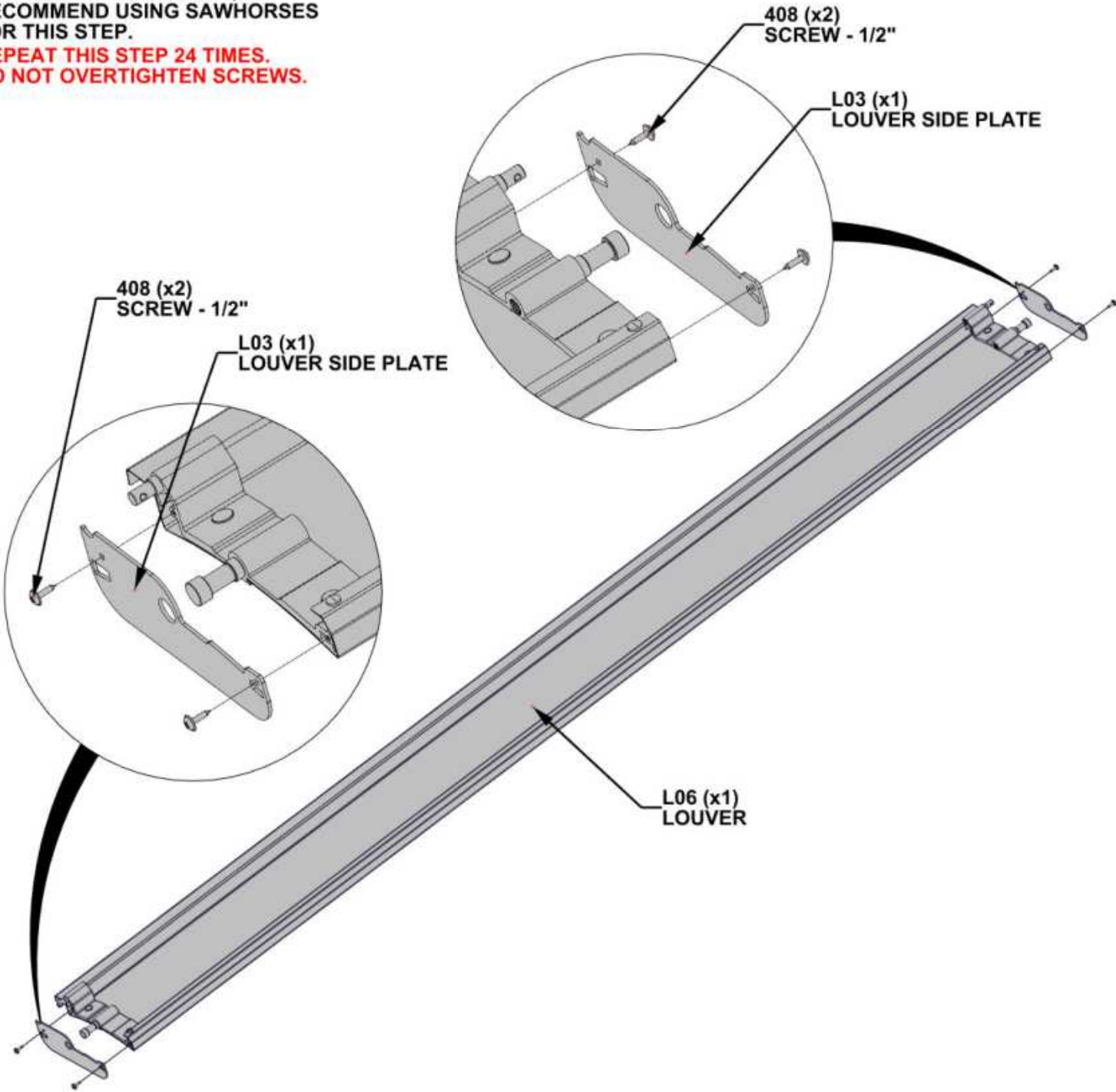
L03 LOUVER SIDE PLATE - A4M04138 (x48) 1/16"x2 3/16"x6 9/16" (2x55x167)
