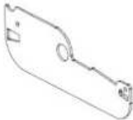
L03 LOUVER SIDE PLATE - A4M04138 (x1) 1/16"x2 3/16"x6 9/16" (2x55x167)
