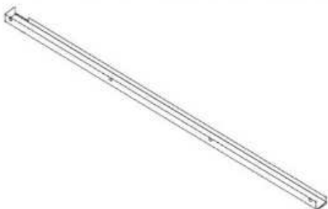
G07 GUTTER - A4M06479 (x1) 1 15/16"x2 11/16"x76 1/2" (50x69x1943)
