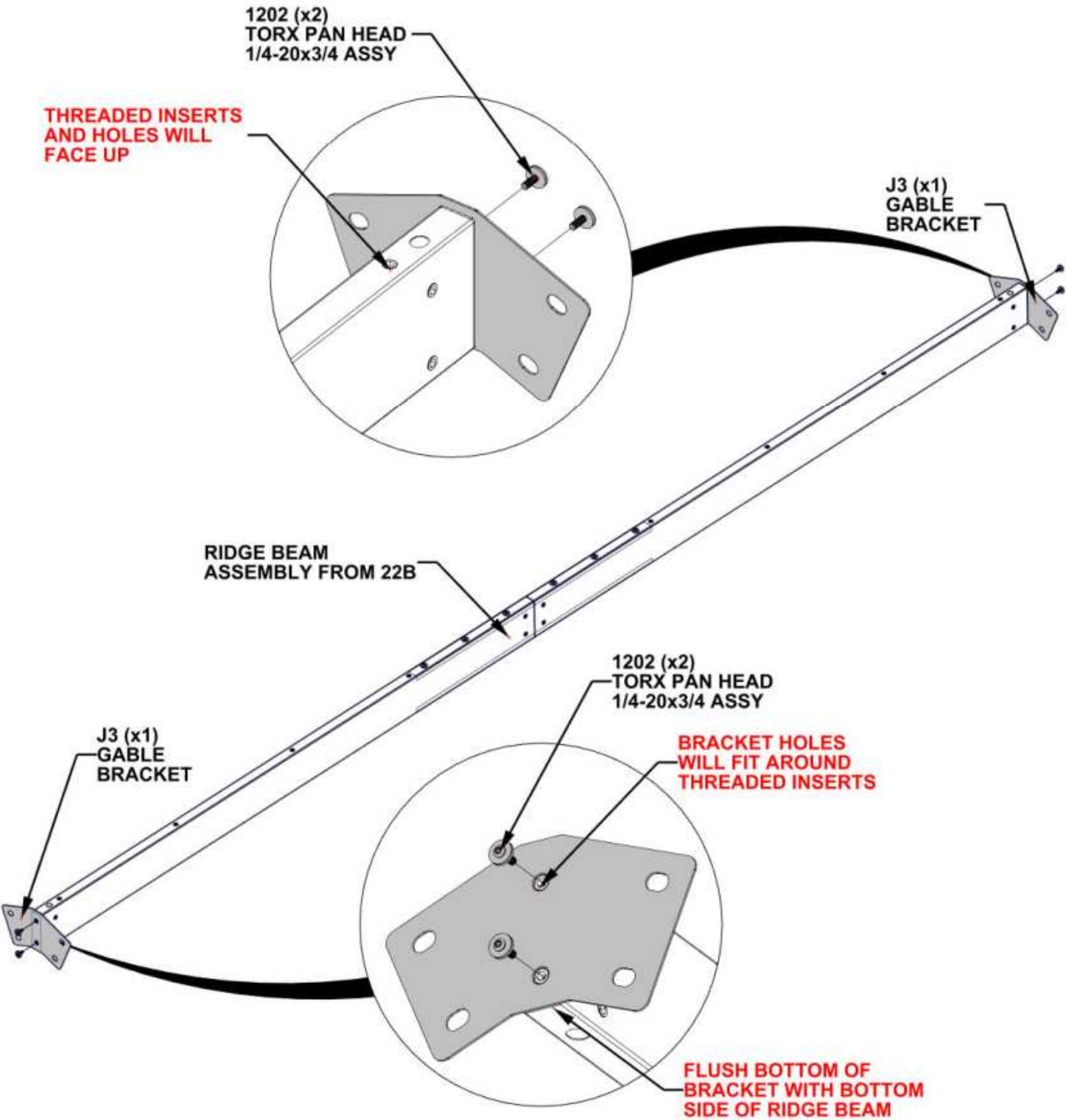
J3 GABLE BRACKET - A4M05824 (x2) 1/16"x6 9/16"x10 15/16" (2x167x277)
