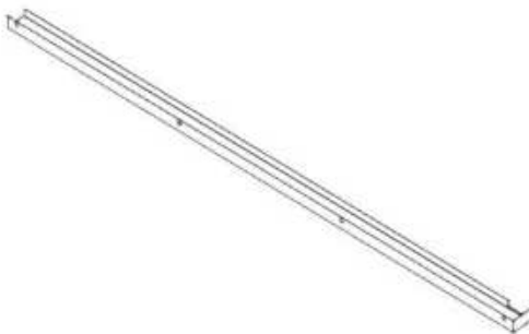
G08 GUTTER - A4M06480 (x2) 1 3/4"x2 11/16"x76 1/2" (50.00x69x1943)
