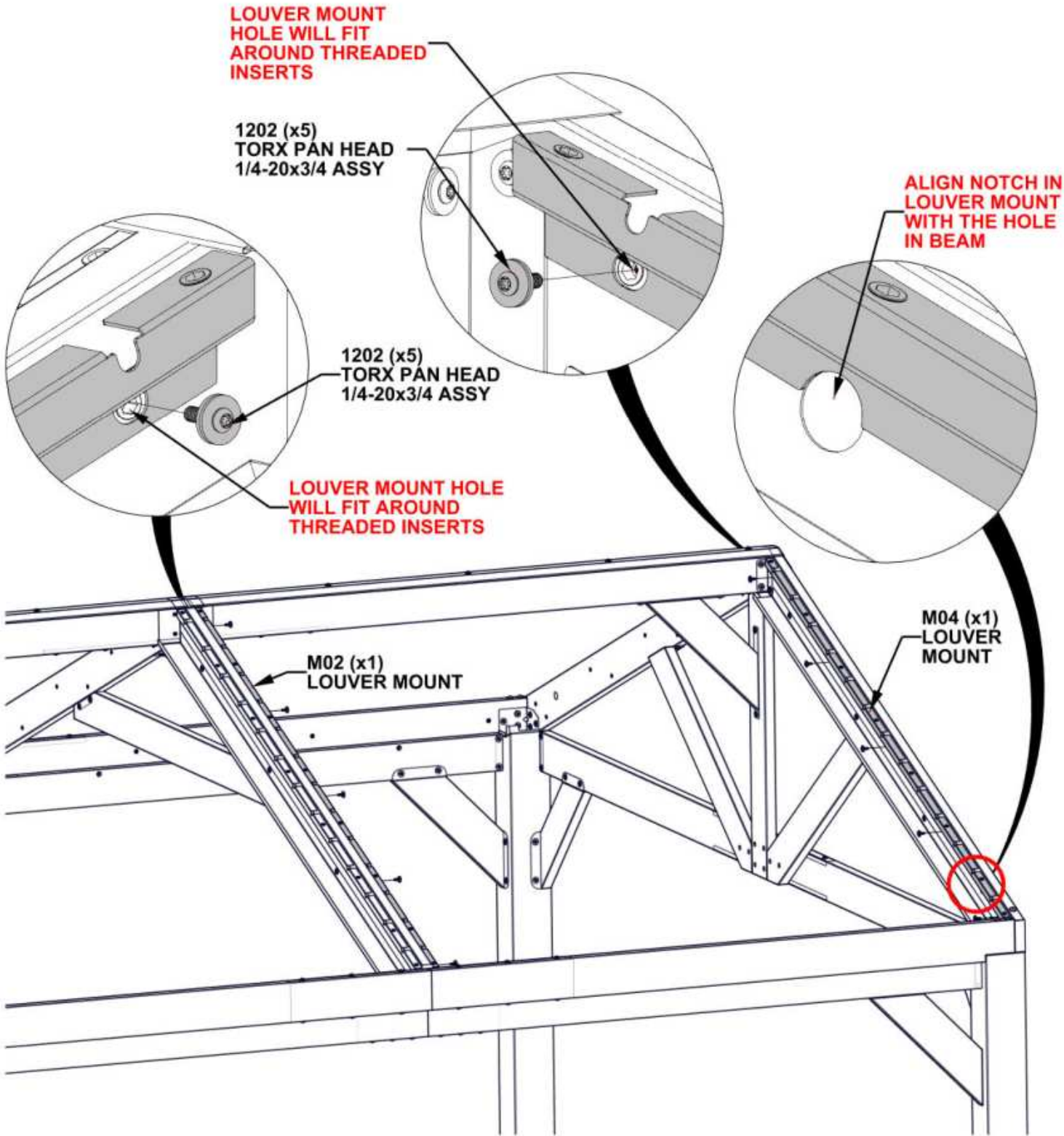
M02 LOUVER MOUNT - A4M05831 (x1) 1"x1 15/16"x88 1/4" (25x49x2241)
