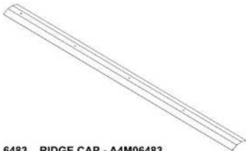
6483 RIDGE CAP - A4M06483 (x2) 3/4"x5 3/8"x82 3/8" (19x137x2093)
