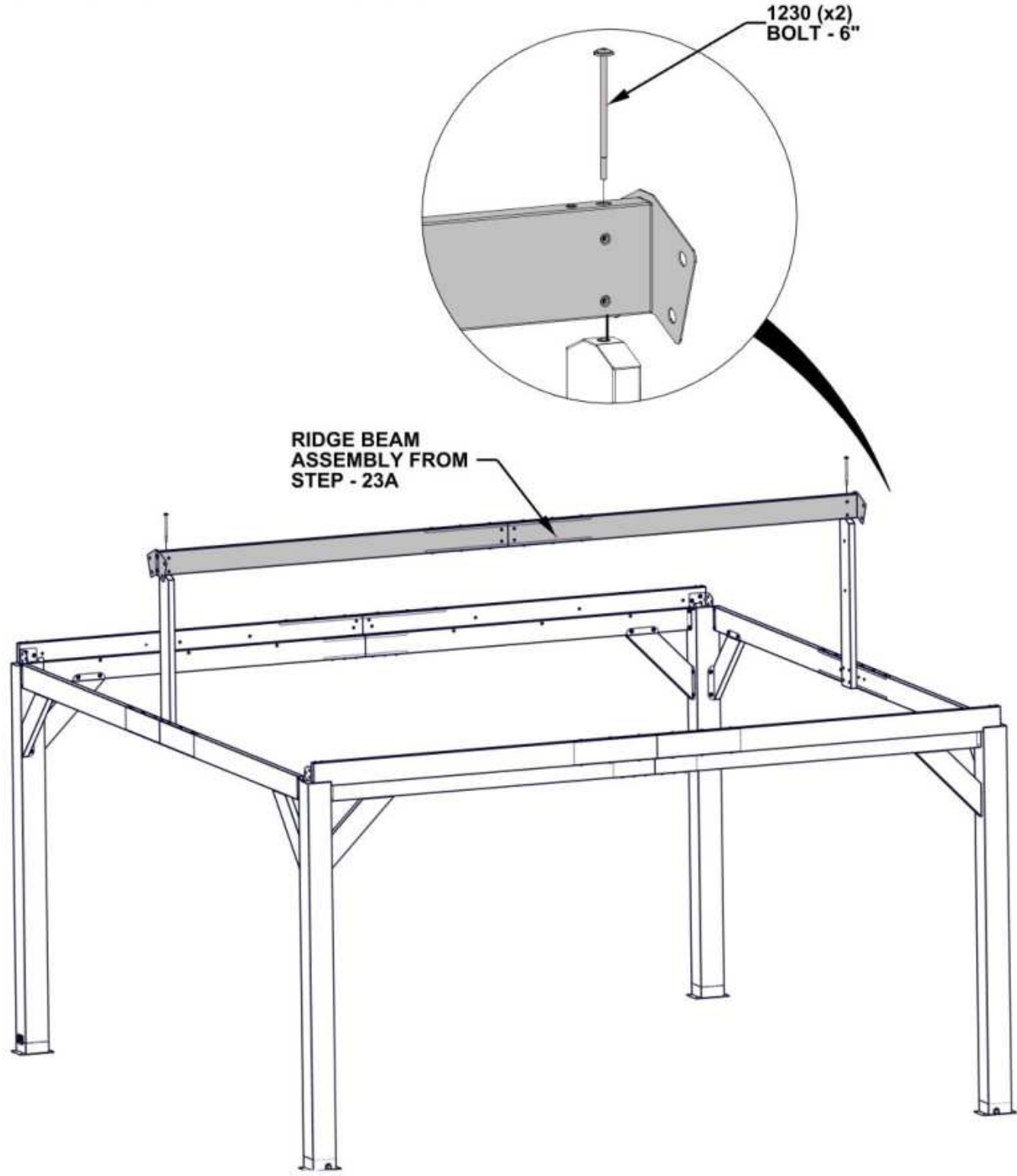
RIDGE BEAM ASSEMBLY FROM STEP - 23A
