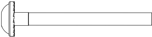
H100999 | BOLT WH (x4) | 1/4 X 2 1/2
