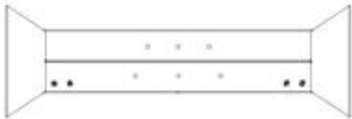
S12 SWING BEAM STRINGER ASSEMBLY - A4M06608 (x1) 34 1/2"x11 1/8"x2 5/8" (88x283x877)
