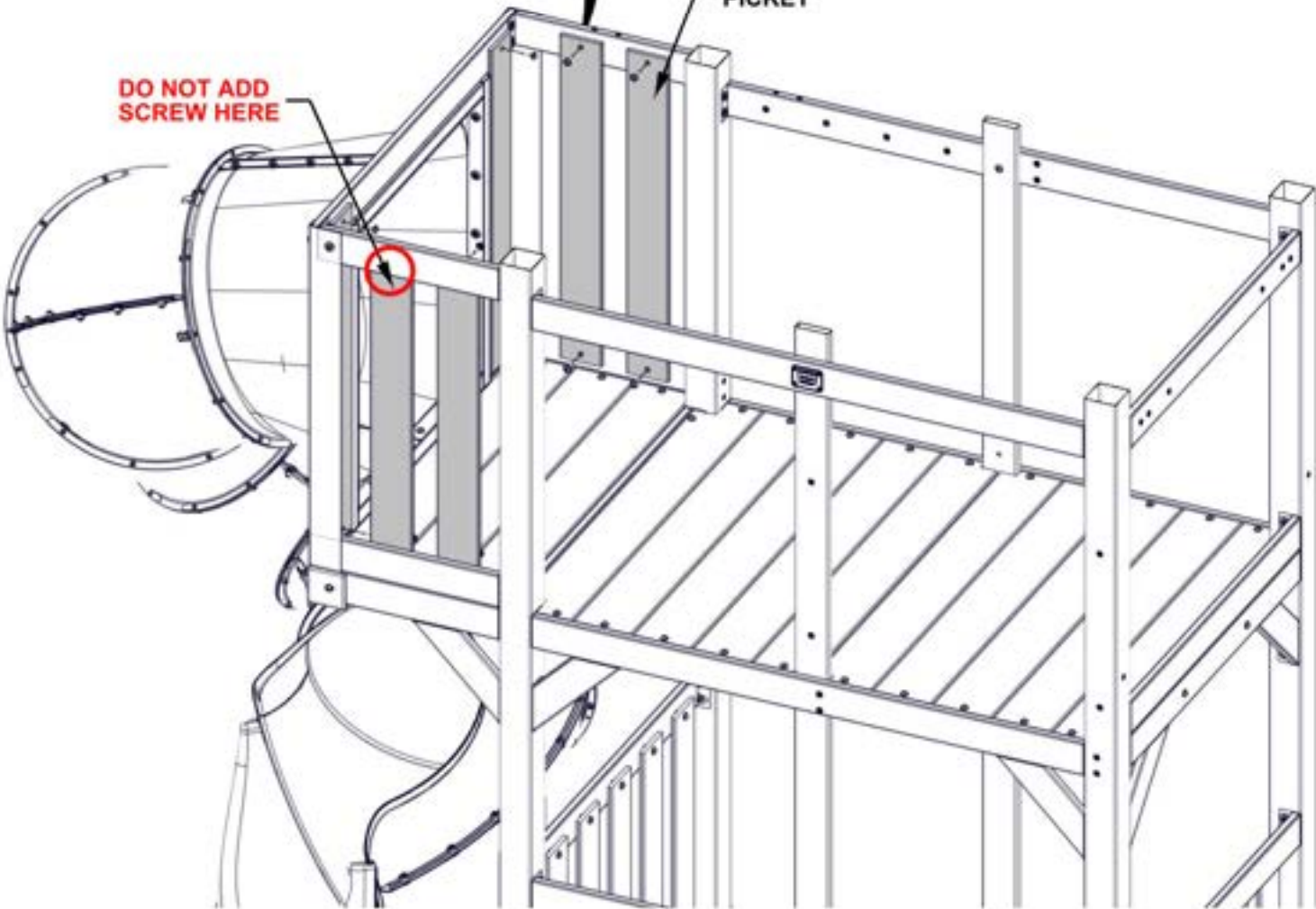
W16 (x6) PICKET
