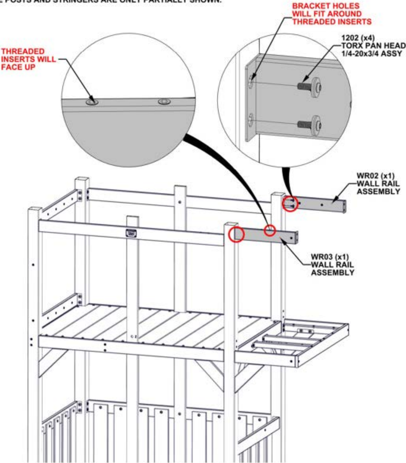
WR03 WALL RAIL ASSEMBLY - A4M05943 (x1) 16 7/8"x3 1/8"x1 15/16" (50x80x429)
