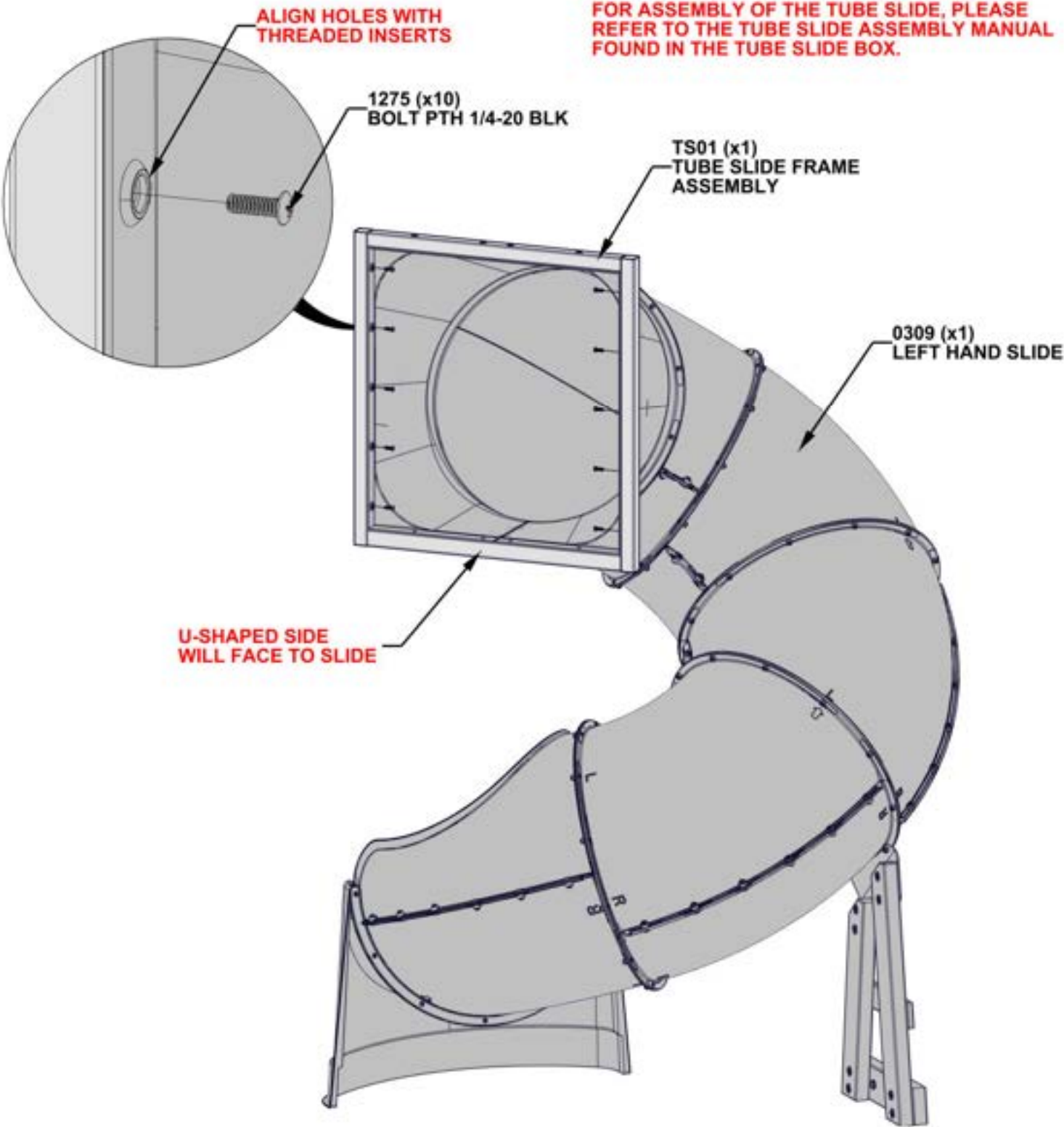
9230309 LEFT HAND SLIDE (x1)
