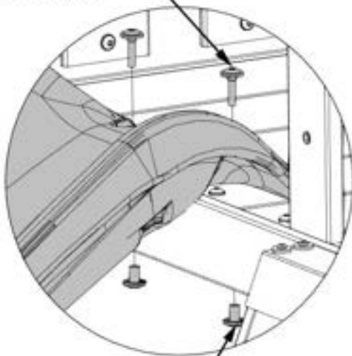
469 (x2) NUT BARREL WH 5/16 X 5/8 BLK
