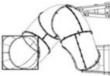
9230309 LEFT HAND SLIDE (x1)
