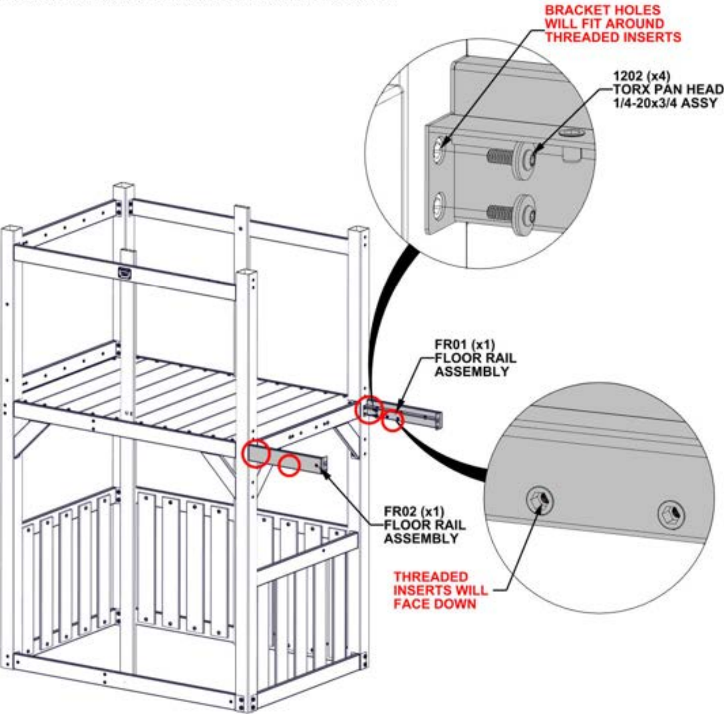
FR02 FLOOR RAIL ASSEMBLY - A4M05937 (x1) 18 1/4"X3 1/8"X1 5/16" (50x80x429)
