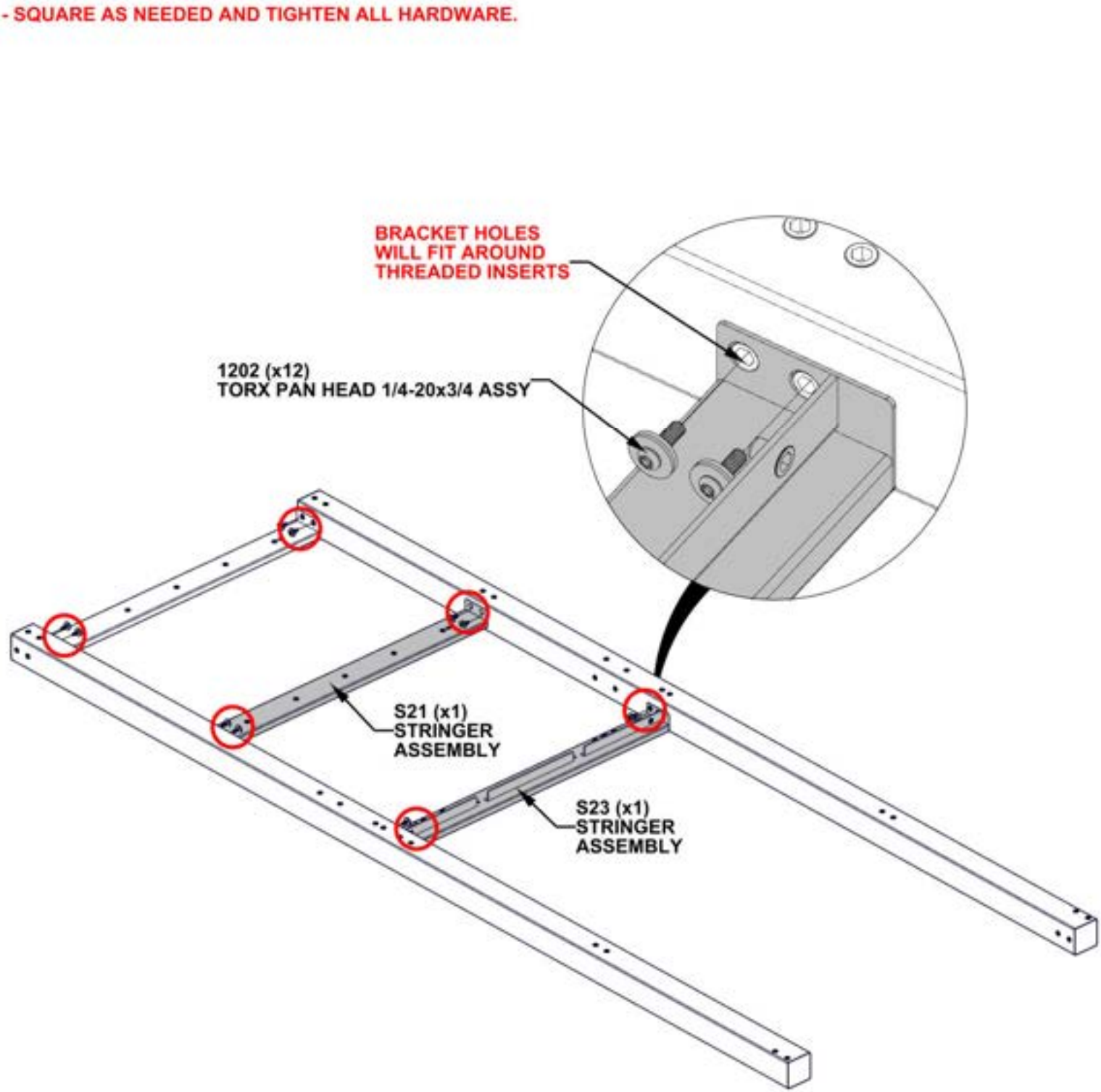
S23 STRINGER ASSEMBLY - A4M07163 (x1) 34 1/2"x3 1/8"x2" (50x80x877)
