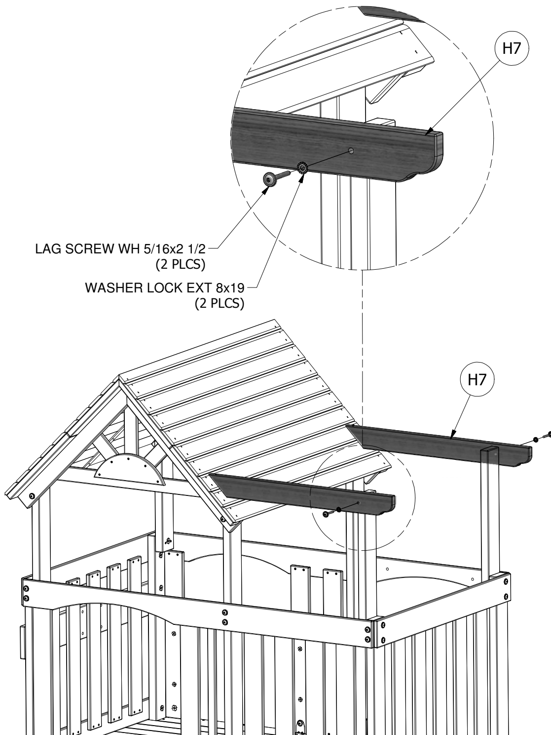
(2) LAG SCREW WH 5/16x2 1/2
