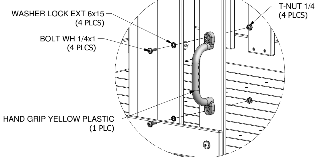
HAND GRIP YELLOW PLASTIC (1 PLC)
