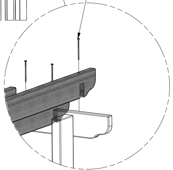
SCREW PFH 8x3 (16 PLCS)
