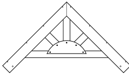
(2) GABLE ASSEMBLY
