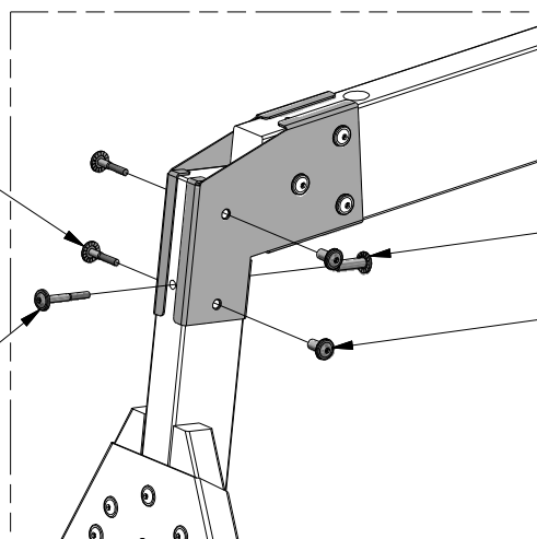
H100011 | BOLT WH (x2) | 5/16x1 3/4
