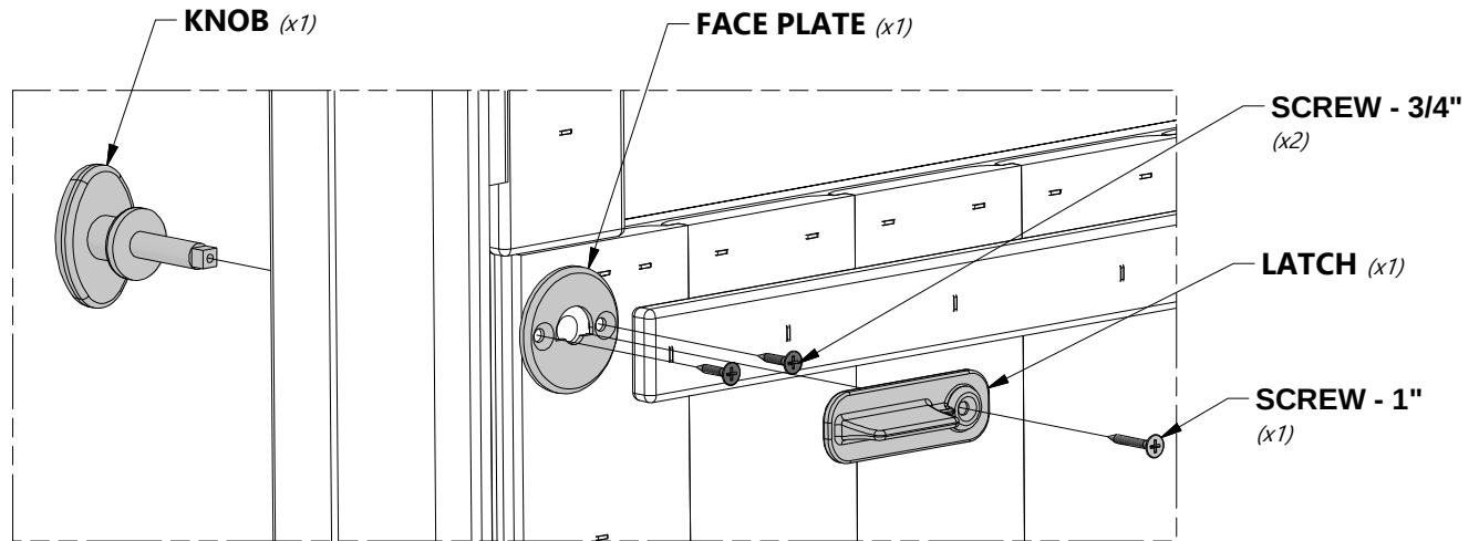
A6P00020 (x1) | LATCHING KNOB KIT
