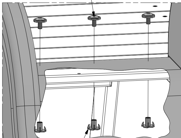
074 (x3) T-NUT - 5/16"
