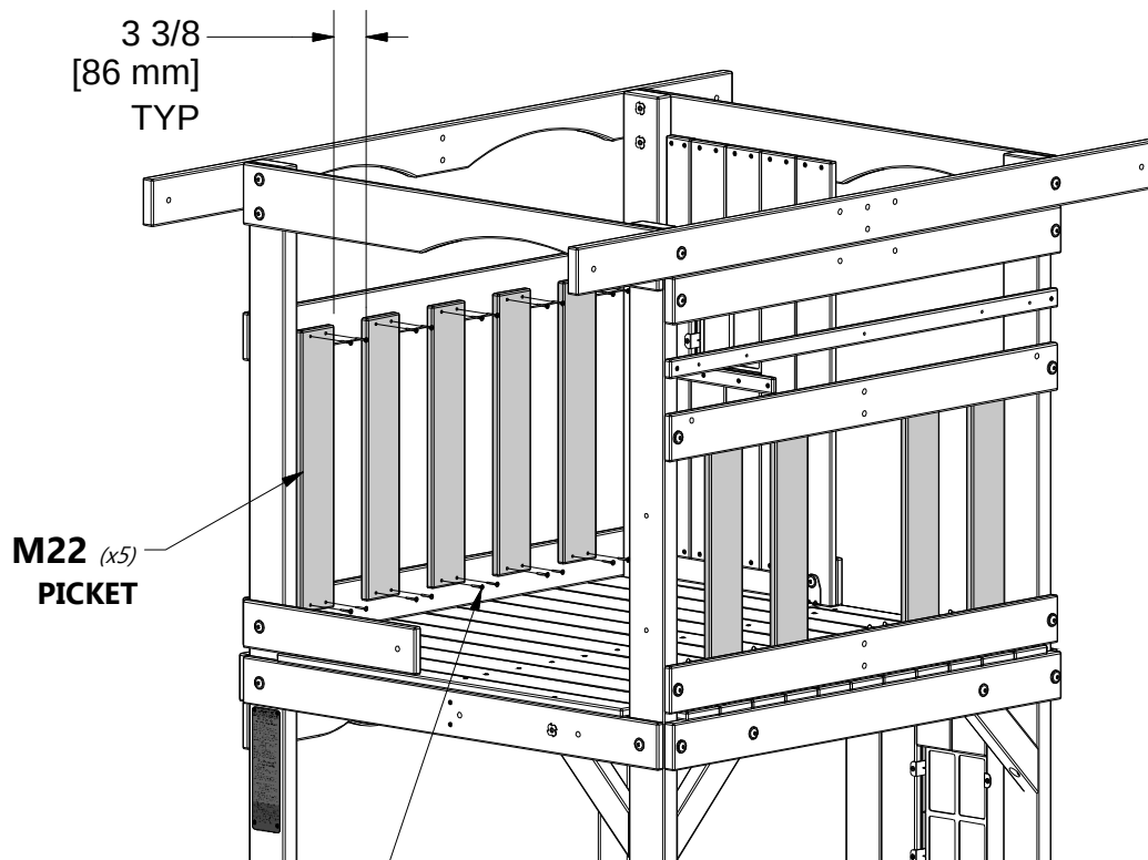
088 (x36) SCREW - 1 1/8"
