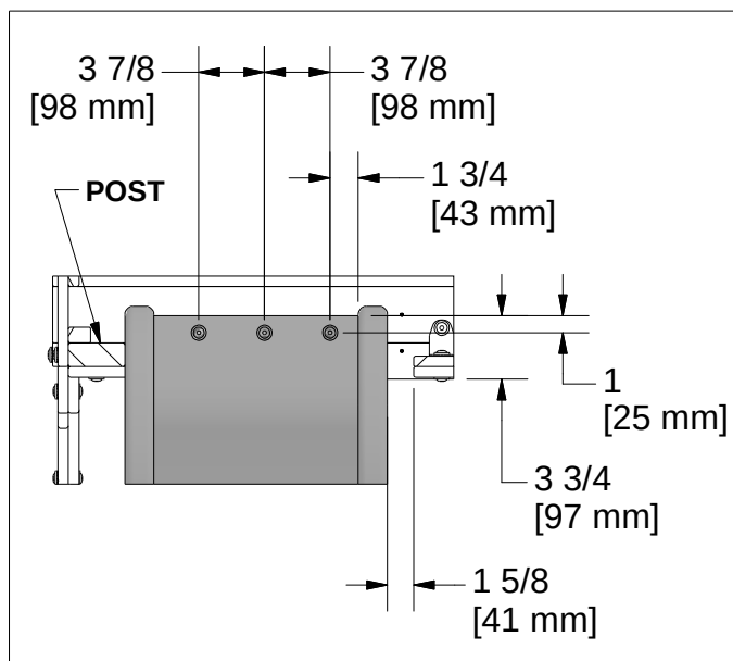
DRILL PATTERN
