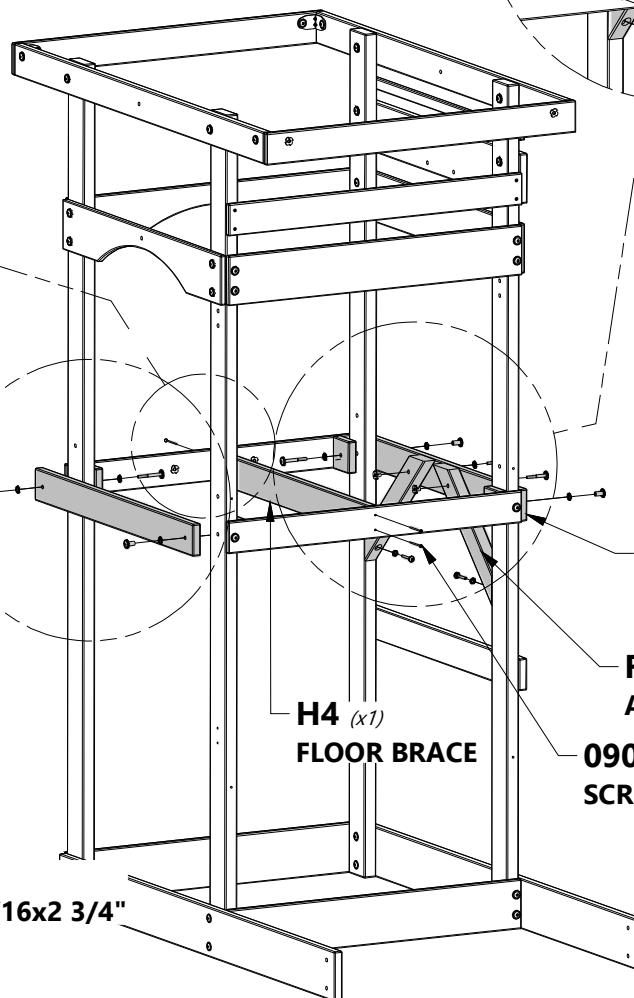
015 (x2) BOLT - 5/16x2 3/4"
