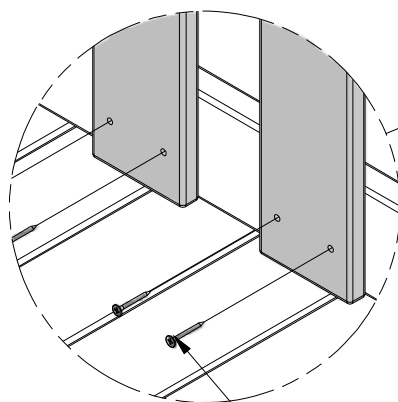
087 (x8) SCREW - 1-1/4"
