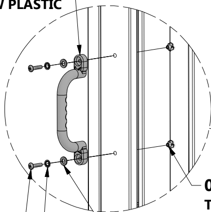
106 (x4) WASHER - 9x18
