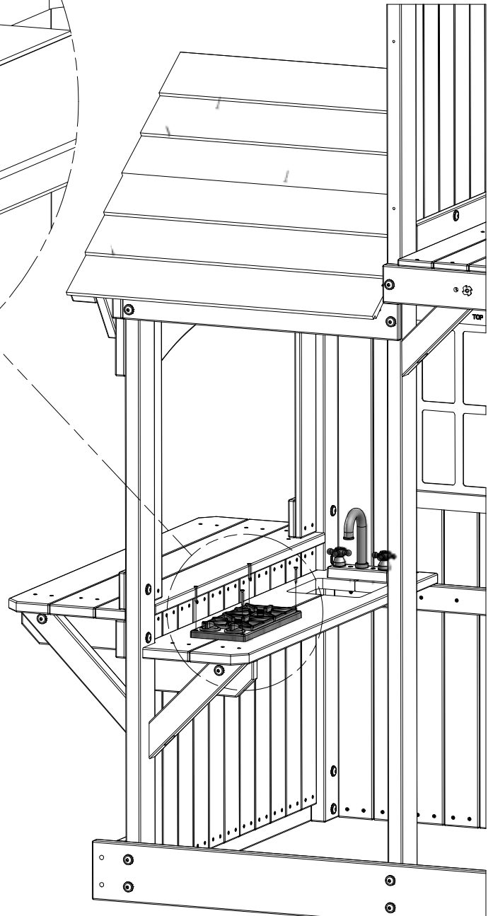
(4) SCREW PFH 8x1 1/2
