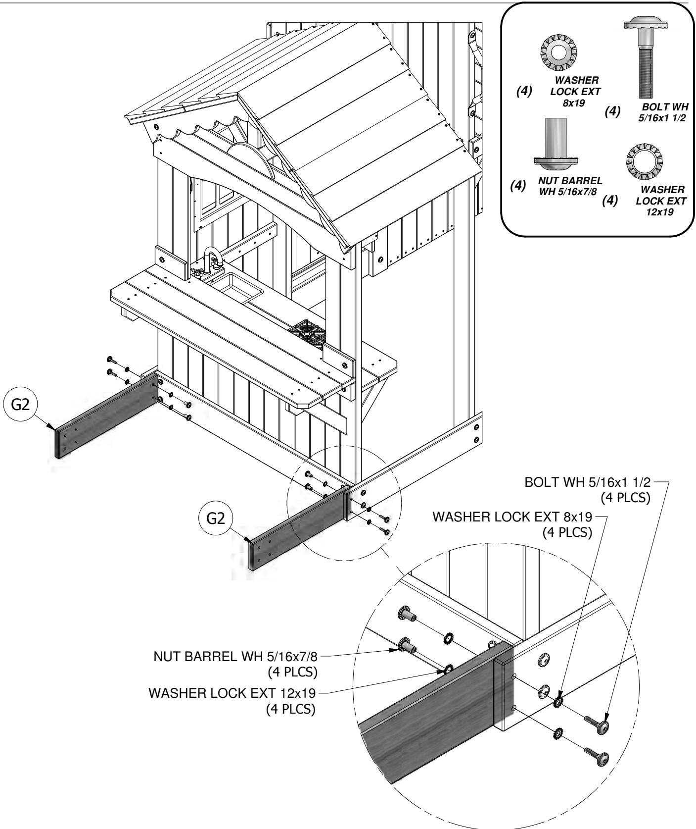
(2) G2 - HORIZONTAL BENCH LEG - W104168 1"x5 1/4"x22" (24x134x560)
