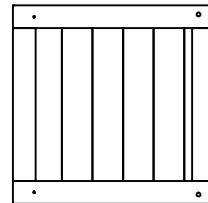
(1) WP7 - RIGHT MIDDLE PANEL - W2A01661 1 1/8"x20 5/8"x21" (27x524x534)
