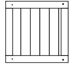
(1) WP7 - RIGHT MIDDLE PANEL - W2A01661 1 1/8"x20 5/8"x21" (27x524x534)
