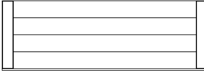
(1) RP3 - PORCH PANEL - W2A01694 1 5/8"x20 5/8"x60 7/8" (42x524x1546)
