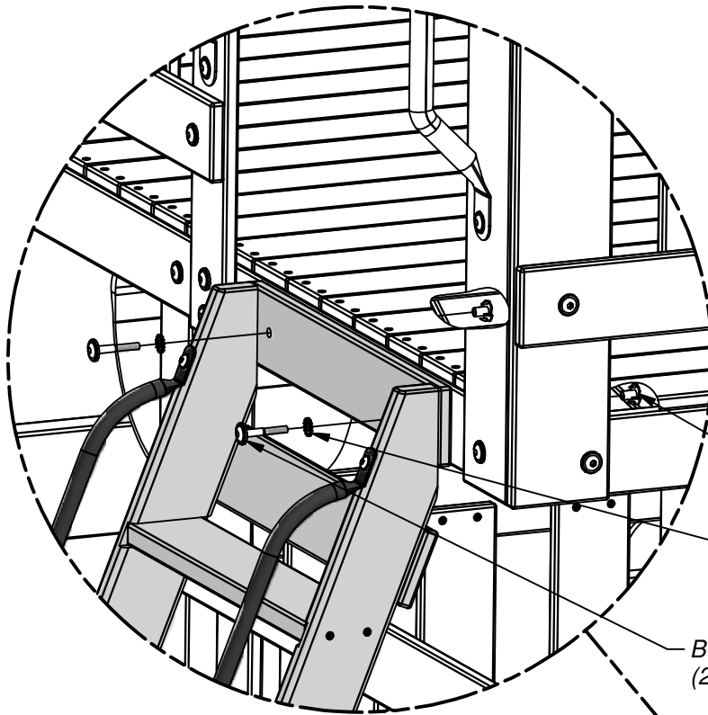
LADDER ASSEMBLY
