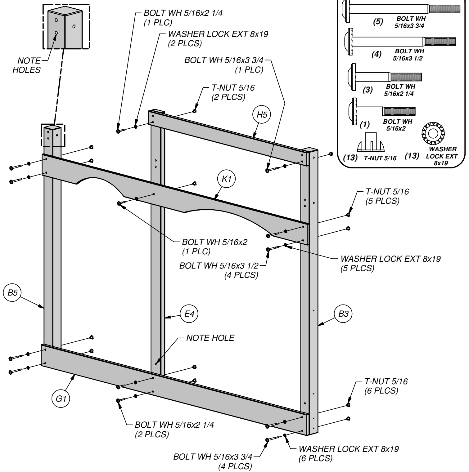
(1) E4 - UPRIGHT - W4L05387 1 3/8"x3 3/8"x70 3/8" (36x86x1786)
