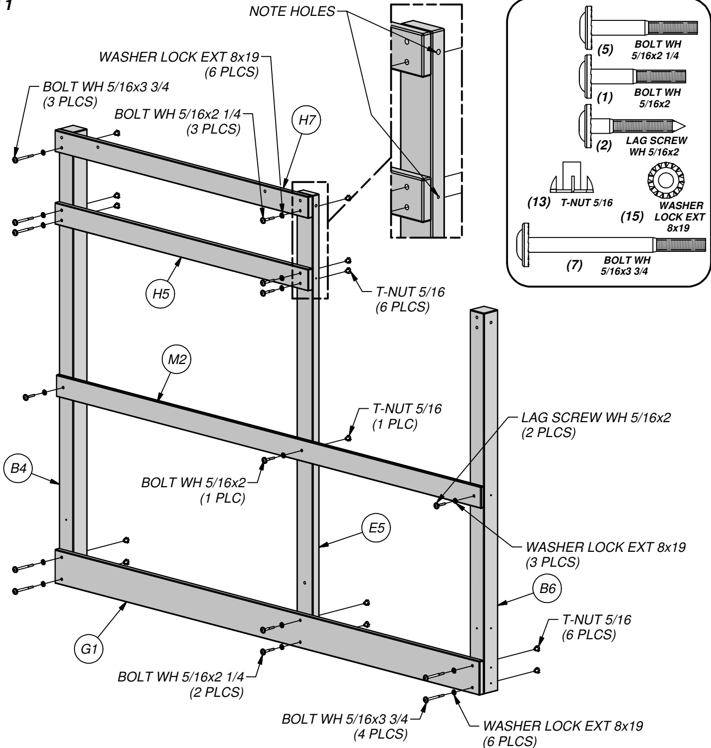
(1) E5 - UPRIGHT - W4L05609 1 3/8"x3 3/8"x70 3/8" (36x86x1786)
